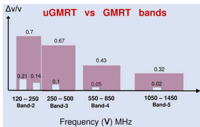
Figure 1. Frequency coverage and fractional bandwidth of the four uGMRT bands being commissioned at present, in comparison with the existing GMRT bands (figure courtesy: Ruta Kale, NCRA).
